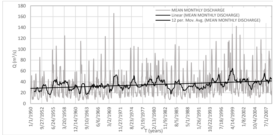
Fig. 2. Visu hydrometric station 1950-2008 mean monthly discharge data
